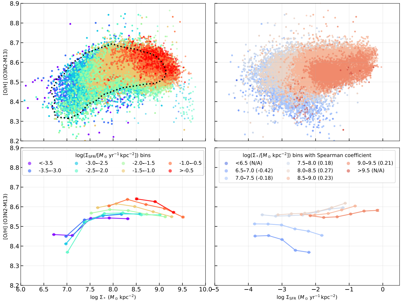
Figure 3. The left column shows the rMZR colour-coded by \Sigma_{\text{SFR}} for 13 MAUVE–MUSE galaxies (excluding NGC 4383), while the right column shows the Z_{\text{gas}}\text{--}\Sigma_{\text{SFR}} relation colour-coded by \Sigma_* . The upper panels display the scatter plots, while the lower panels show the corresponding median trends of each scatter plot. Similar to Figure 2, we use the black contour to enclose the 95% population of HII spaxels. Within this contour, we present the median trends with errorbars indicating the standard error of the median (SEM; typical value of \lesssim 0.01 ). Note that due to insufficient statistics, the median trends of the lowest and highest \Sigma_* bins in the bottom right panel are not shown.
